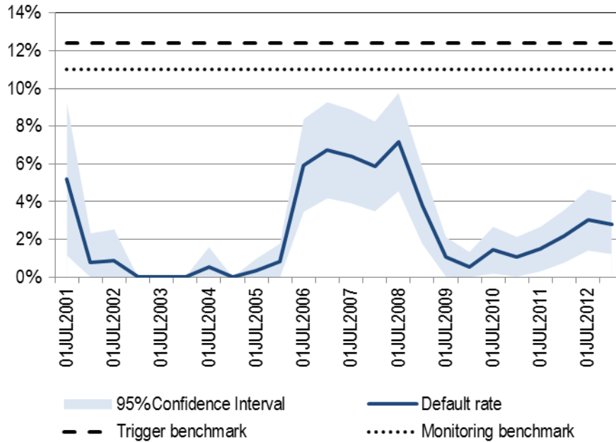
Figure 16: Short-run and long-run observed default rates of BB rating category
