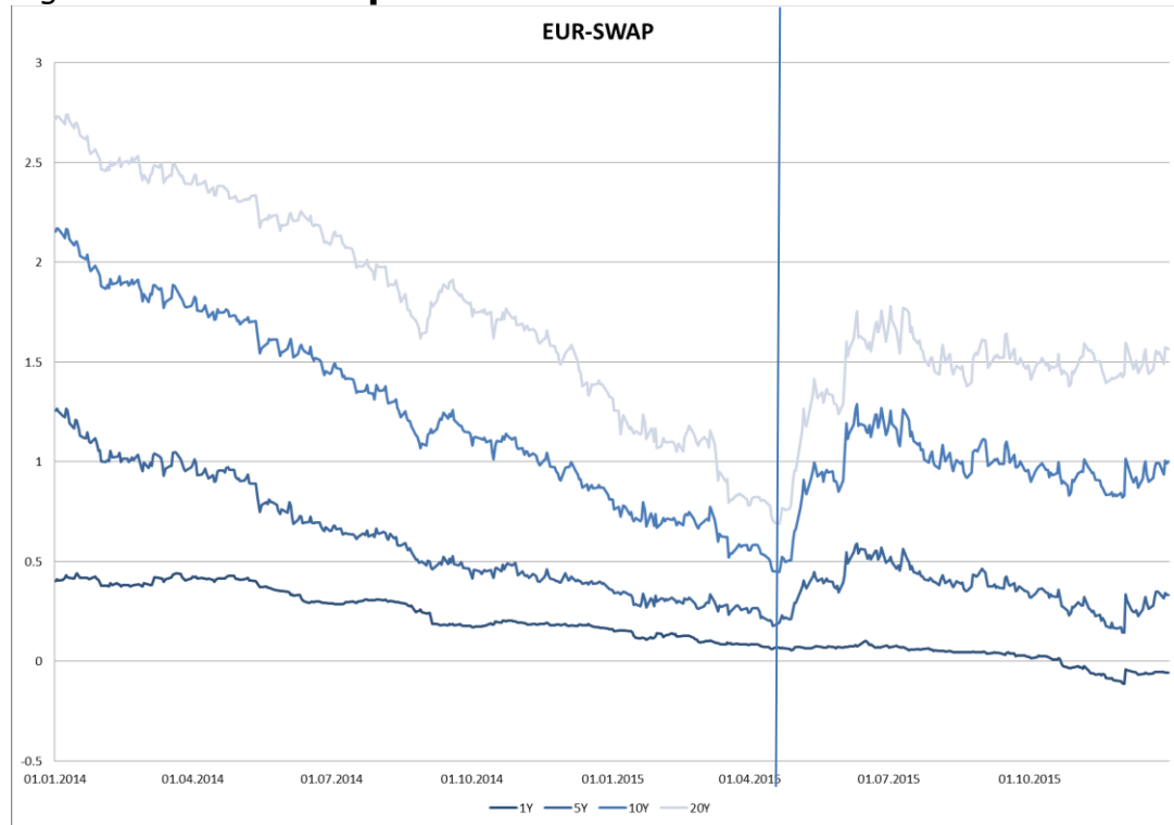
Figure 1– Euro-Swap curve
