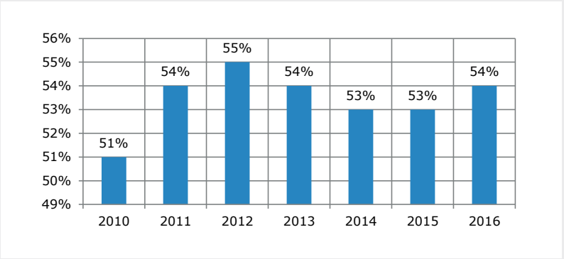
Figure B2: Percentage of transitional provisions using immunisation techniques
