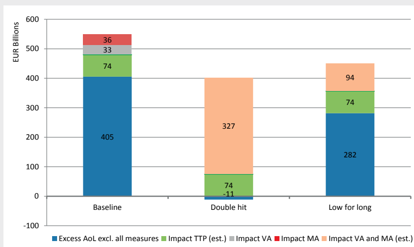
Figure A3: Impact of LTG and transitional measures assuming constant transitionals
