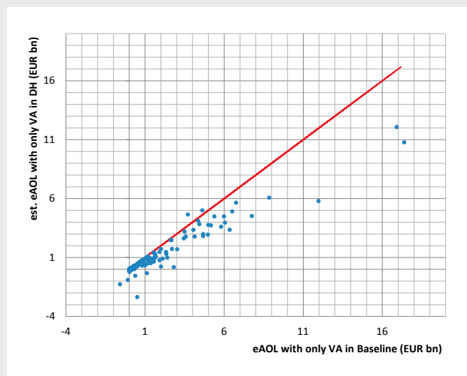
Figure A6: EAOL in baseline versus post-stress only allowing VA
