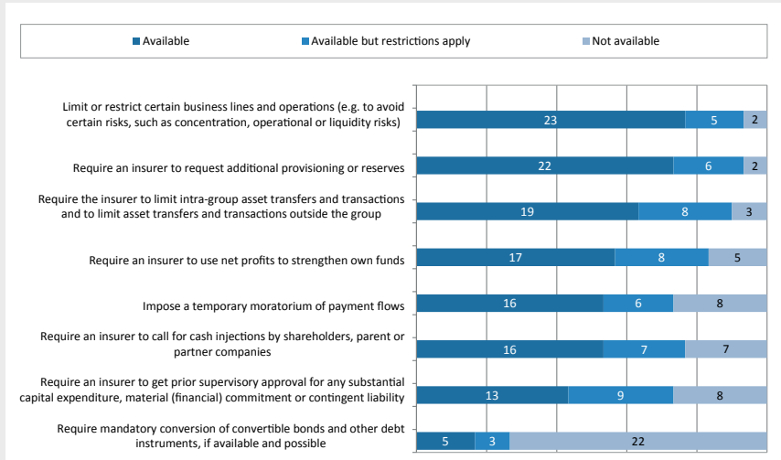
Figure 10: Some additional powers available to NSAs
